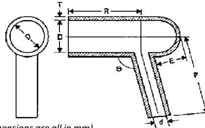
*Drawing depicts typical dimensions (Dimensions are all in mm)
