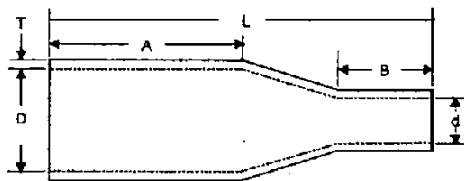
*Drawing depicts typical dimensions (Dimensions are all in mm)
