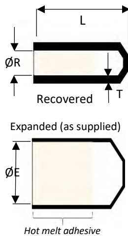
*Drawing shows typical parts
